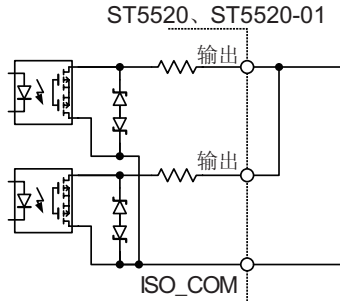
WIRED OR
